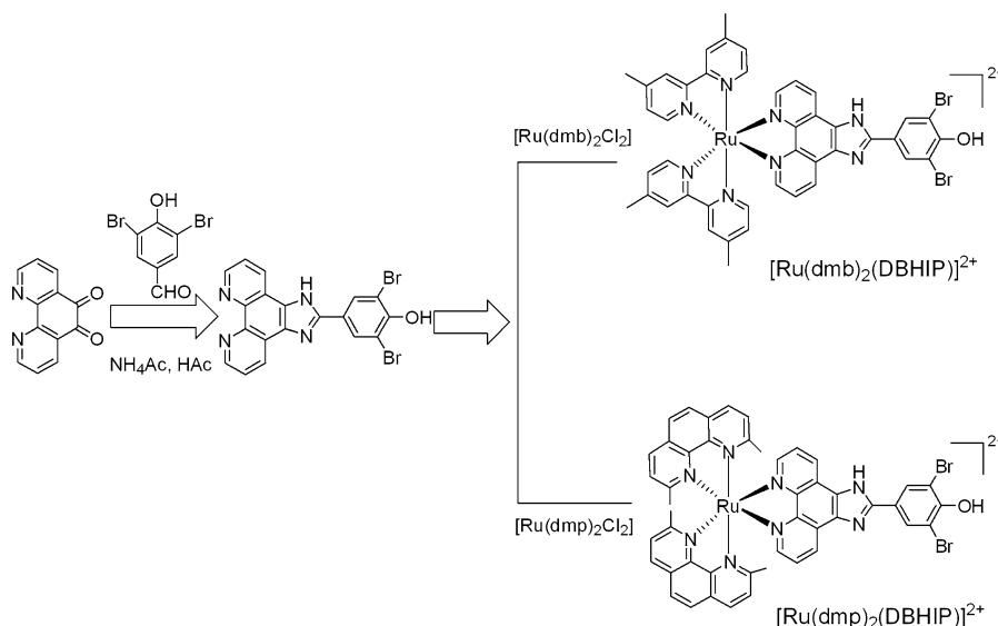
Scheme 1 The synthetic route for ligand and complexes
