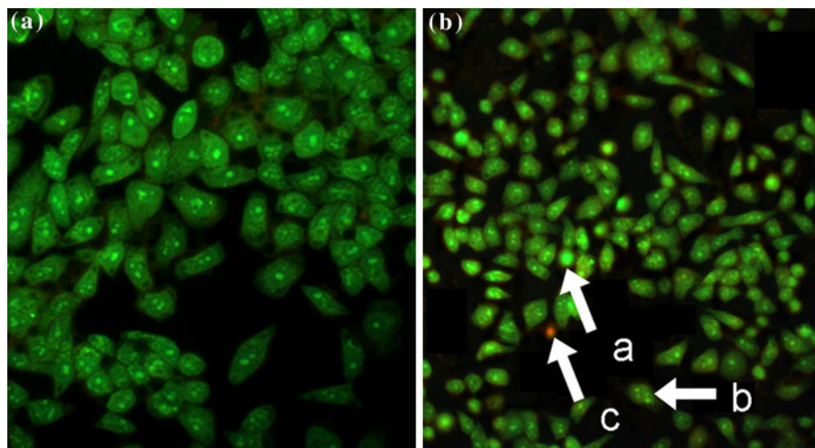
Fig. 7 BEL-7402 cell were stained by AO/EB and observed under fluorescence microscopy. BEL-7402 cell without treatment ( a ) and in the presence of complex 2 ( b ) incubated at
