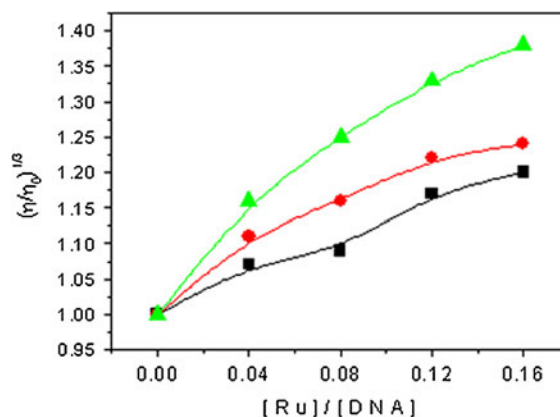
Fig. 1 Effect of increasing amounts of complexes EB (filled triangle), 1 (filled circle) and 2 (filled square) on the relative viscosity of calf thymus DNA at 25 ( \pm 0.1 )°C. [DNA] = 0.30 mM
