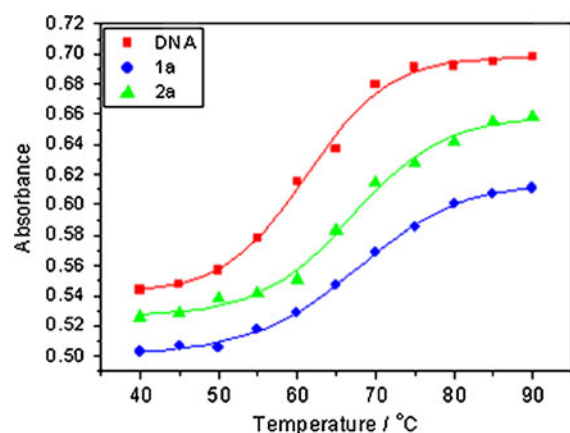
Fig. 3 Thermal denaturation of CT-DNA in the absence (filled square) and presence of complexes 1 (filled circle) and 2 (filled triangle). [Ru] = 32 \mu M, [DNA] = 80 \mu M
