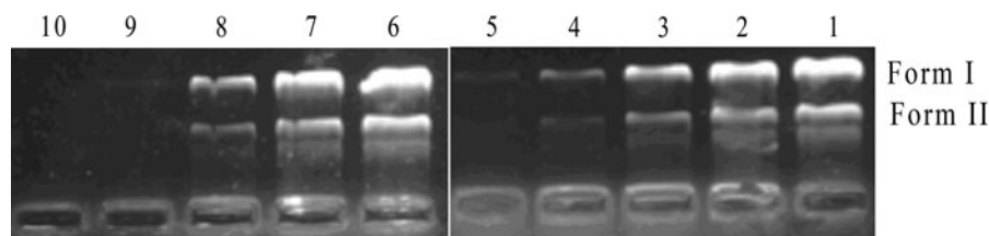
Fig. 5 Agarose gel electrophoresis retardation of pGL 3 plasmid DNA in the presence different concentrations of complexes 1 and 2 . 1: Lane (1) DNA alone, (2) 0.33 mM; (3)
