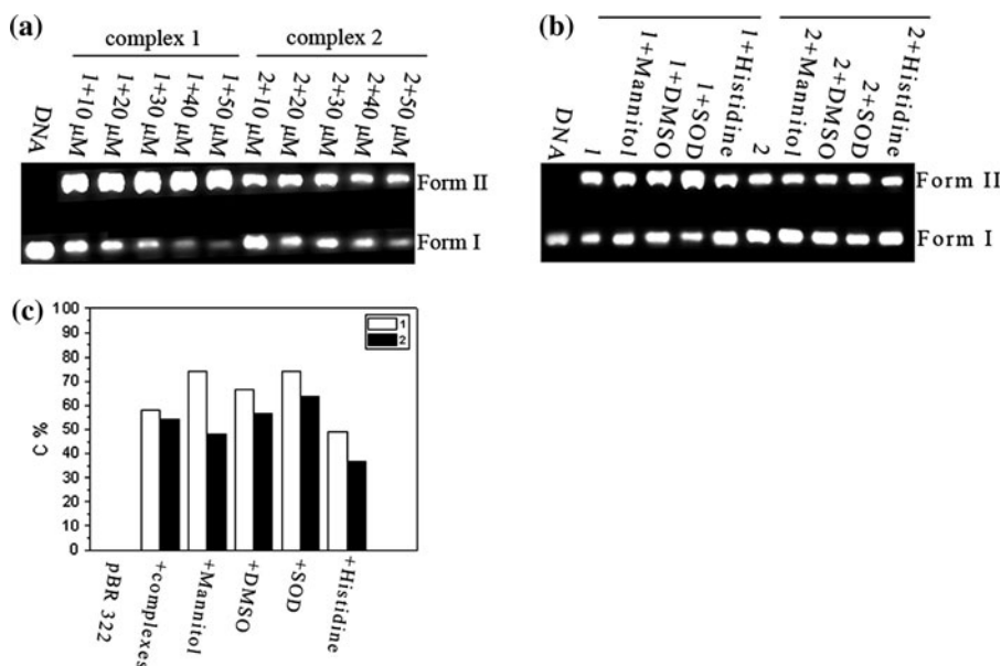
Fig. 4 a Photoactivated cleavage of pBR 322 DNA in the presence of different concentrations of Ru(II) complexes after irradiation at 365 nm for 30 min. b Photoactivated cleavage of supercoiled pBR 322 DNA by complexes 1 and 2 (20 \mu\text{M} ) in the absence and presence of different inhibitors [100 mM
