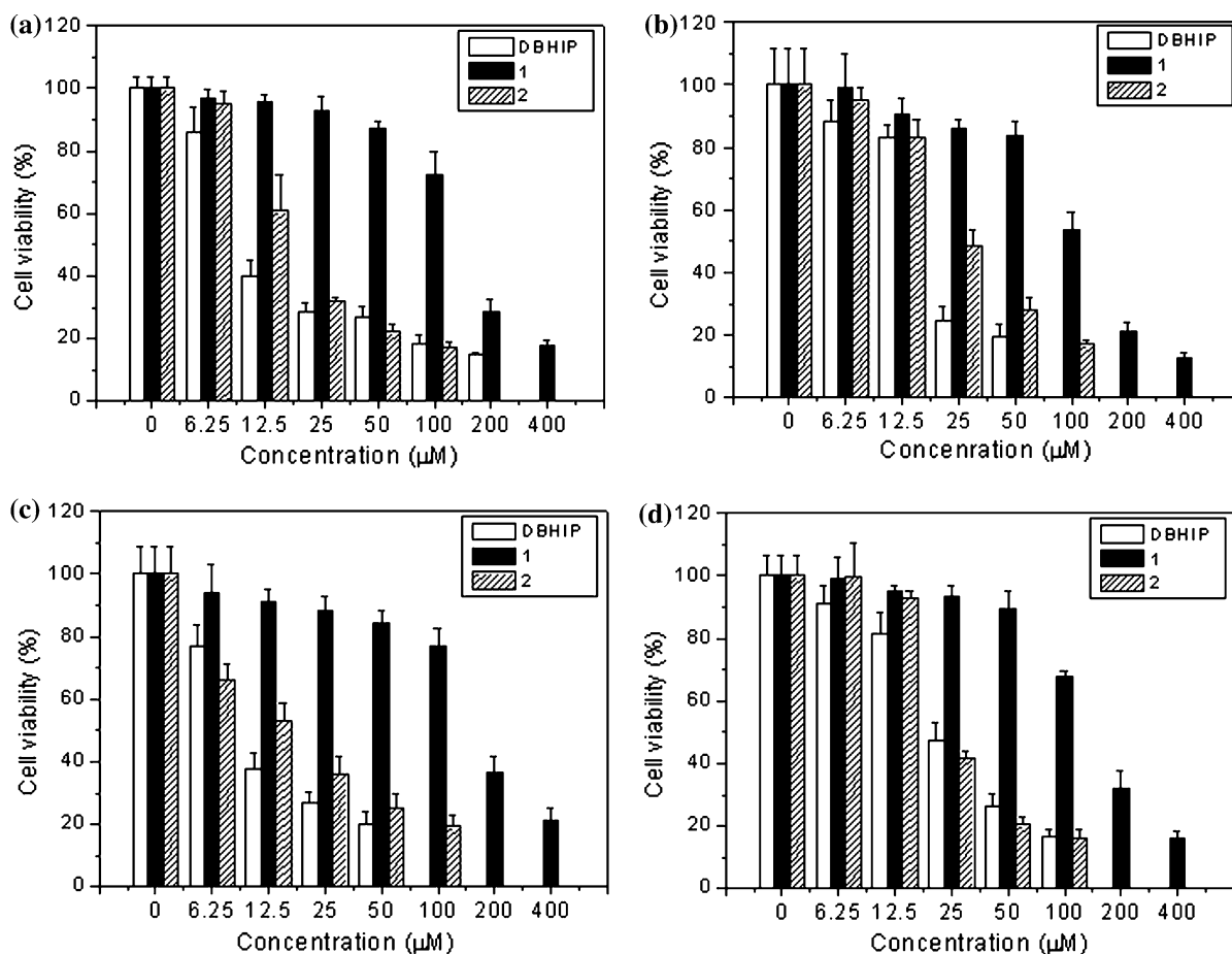
Fig. 6 a Cell viability of DBHIP, 1 and 2 on tumor BEL-7402 ( a ), C-6 ( b ), HepG-2 ( c ) and MCF-7 ( d ) cell proliferation in vitro. Each data point is the mean ± standard error obtained from at least three independent experiments. b Light microscopy of C-6 cell line after treated for 48 h in the absence I
