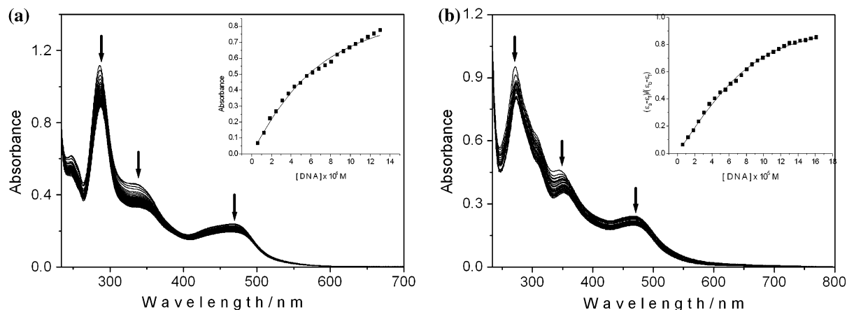
Fig. 2 Absorption spectra of complexes 1 (a) and 2 (b) in Tris-HCl buffer upon addition of CT-DNA. [Ru] = 20 \mu M. Arrow shows the absorbance change upon the increase of DNA
