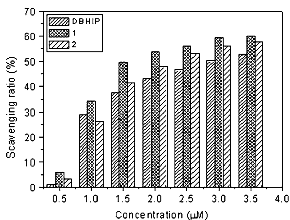
Fig. 8 Scavenging effect of the ligand DBHIP and complexes 1 and 2 on hydroxyl radicals. Experiments were performed in triplicate
